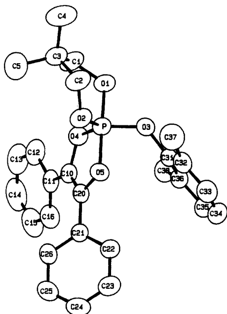
Figure 1. ORTEP plot of (\text{Me}_2\text{C}_3\text{H}_4\text{O}_2)(\text{Xyl-O})\text{P}(\text{O}_2\text{C}_2\text{Ph}_2) ( 1 ) with thermal ellipsoids at the 50% probability level. Hydrogen atoms are omitted for clarity.
