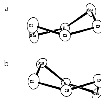
Figure 6. ORTEP plot showing the boat conformations of the six-membered phosphorane rings in 4 : (a) showing the A set of positions for the oxygen atoms and (b) showing the B set of positions for the oxygen atoms. The pseudo mirror plane which takes one set of oxygen atoms into the other and C1 into C2 passes through P and C3.
