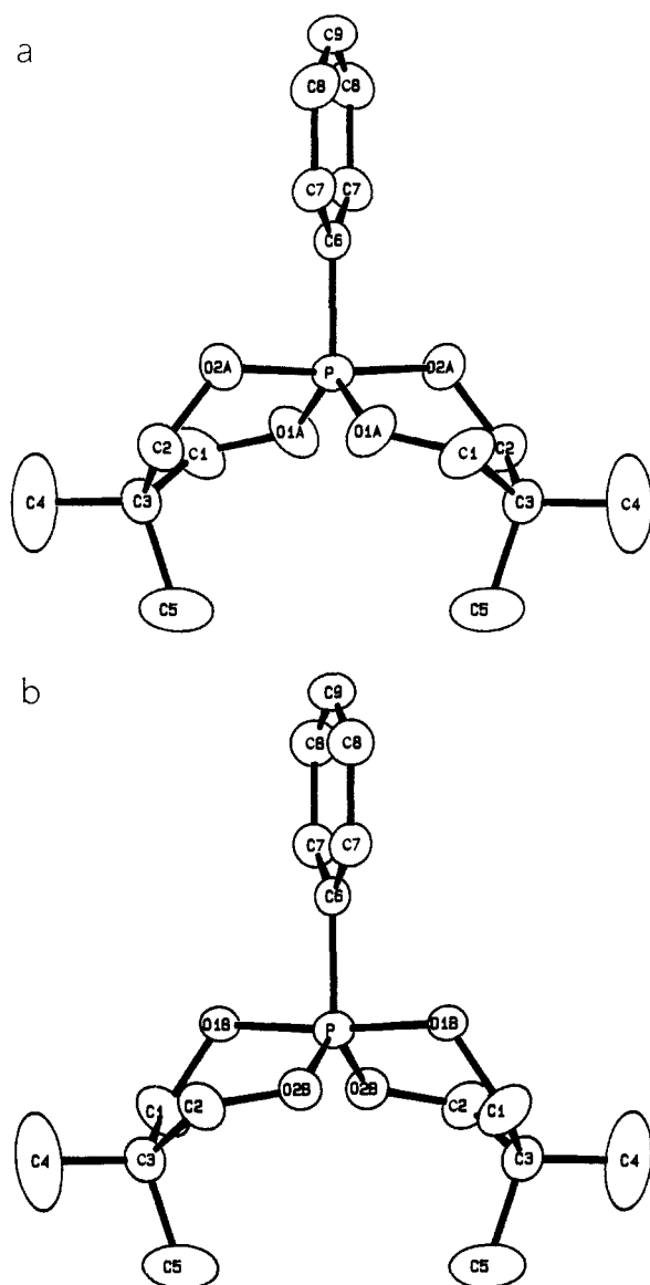
Figure 5. ORTEP plot of (\text{Me}_2\text{C}_3\text{H}_4\text{O}_2)_2\text{PPh} ( 4 ) with thermal ellipsoids at the 30% probability level. Atoms within a molecule with the same label are related by a crystallographic two-fold axis (-x, y, 1/2 - z) : (a) showing the A set of positions for the oxygen atoms and (b) showing the B set of positions for the oxygen atoms.
