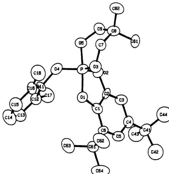
Figure 2. ORTEP plot of (\text{Me}_2\text{C}_3\text{H}_4\text{O}_2)(\text{Xyl-O})\text{P}(\text{O}_2\text{C}_6\text{H}_2-t\text{-Bu}_2) ( 2 ) with thermal ellipsoids at the 50% probability level. The isotropically refined C42, C43, and C44 are represented as spheres of arbitrary radius. Hydrogen atoms are omitted for clarity.
