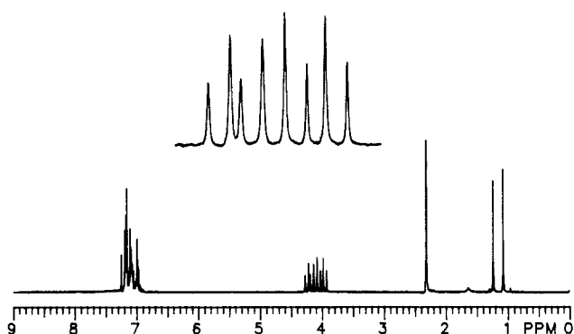
Figure 8. 1 H NMR spectrum of 1 in CDCl 3 at 20 °C. Proton signals from the methyl groups of the phosphorinane ring appear at 1.07 and 1.24 ppm and from the methyl groups of the xylyloxy group at 2.32 ppm. Multiplets appear at 4.00 and 4.21 ppm for the methylene protons of the phosphorinane ring and at 6.90–7.30 ppm for the aromatic protons.
