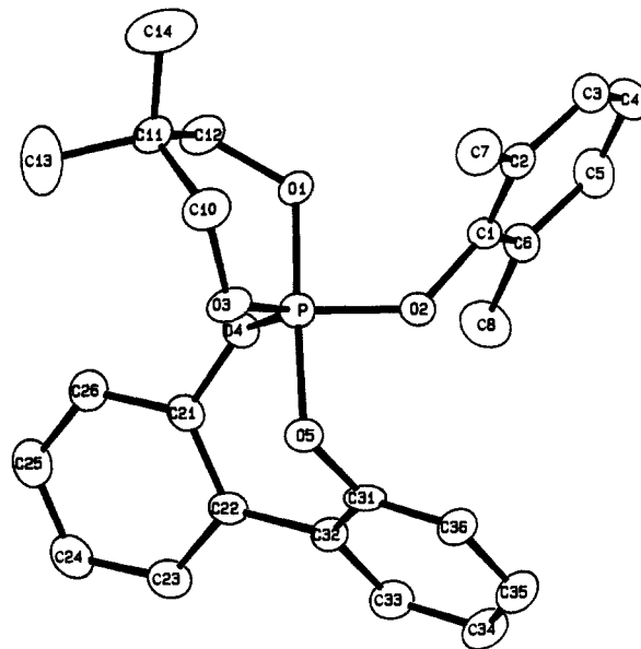
Figure 3. ORTEP plot of the (\text{Me}_2\text{C}_3\text{H}_4\text{O}_2)(\text{Xyl-O})\text{P}(\text{O}_2\text{C}_{12}\text{H}_8) moiety in 3 with thermal ellipsoids at the 30% probability level. Hydrogen atoms are omitted for clarity.
