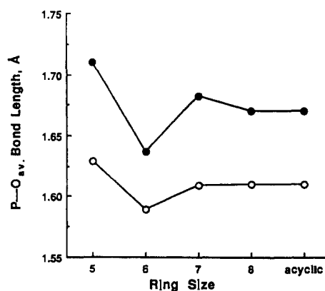
Figure 7. Average P–O bond length vs ring size for apical bonds (filled circle) and equatorial bonds (open circle) obtained from phosphoranes 1–3 and 8–11 , excluding the six-membered ring for 10 .
