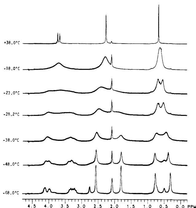
Figure 10. Partial 1 H NMR spectra of 3 as a function of temperature. Additional signals of possibly another isomer appear at 0.48, 0.77, and 2.75 ppm (-68 °C). The peak at 2.1 ppm is due to toluene- d 8 .
